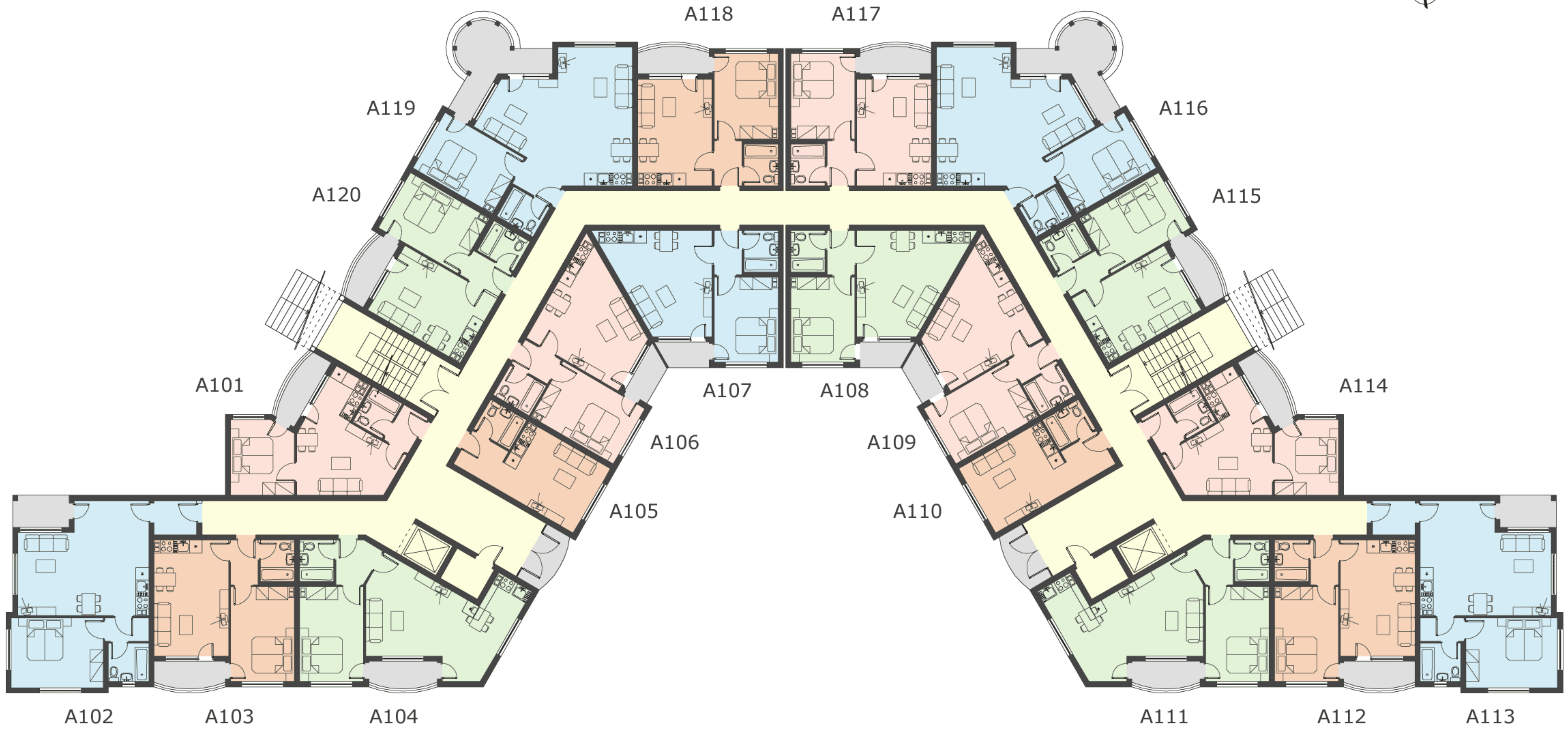
Block A, floor 1 (±0.00)
