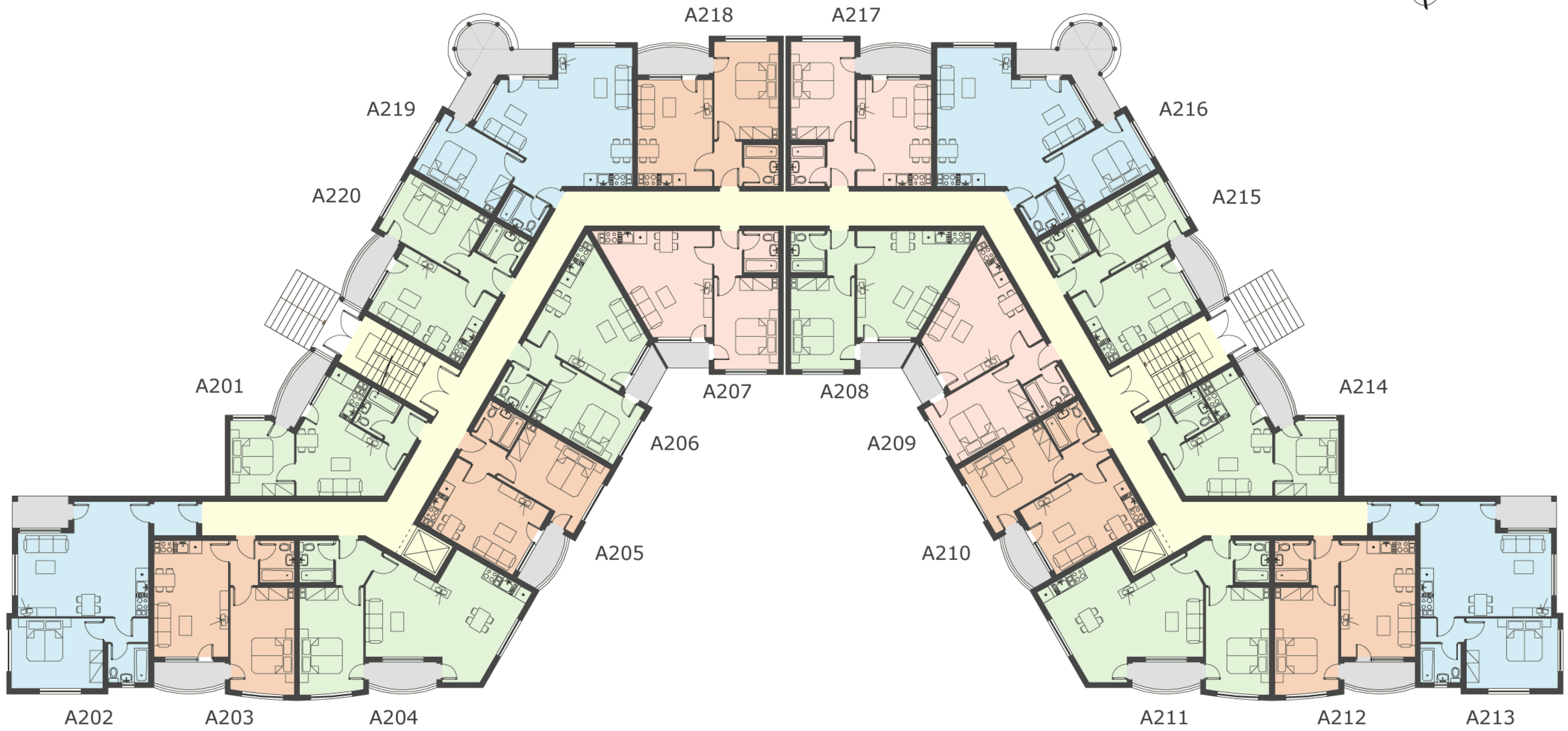
Block A, floor 2 (+2.80)
