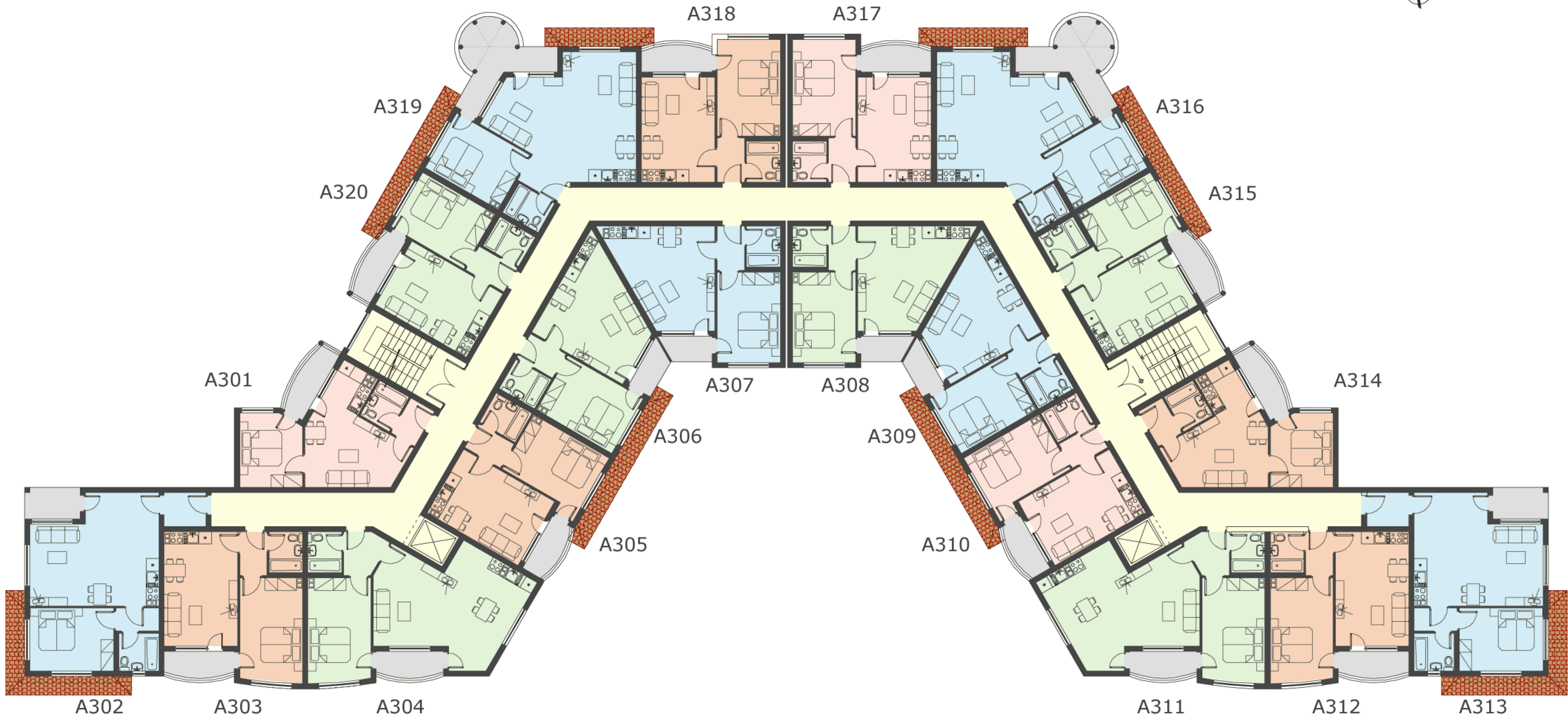
Block A, floor 3 (+5.60)
