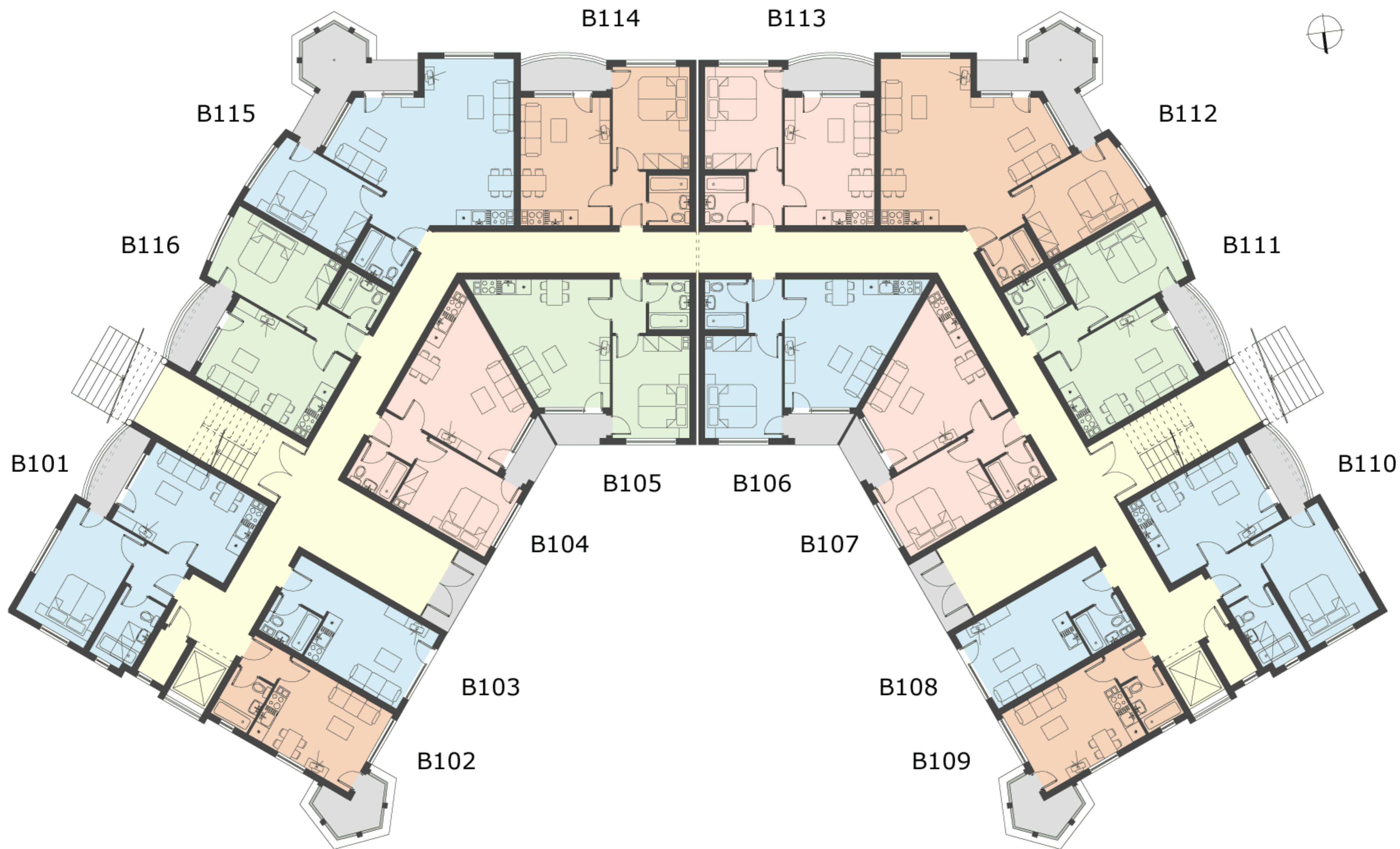
Block BI, floor 1 (±0.00)
