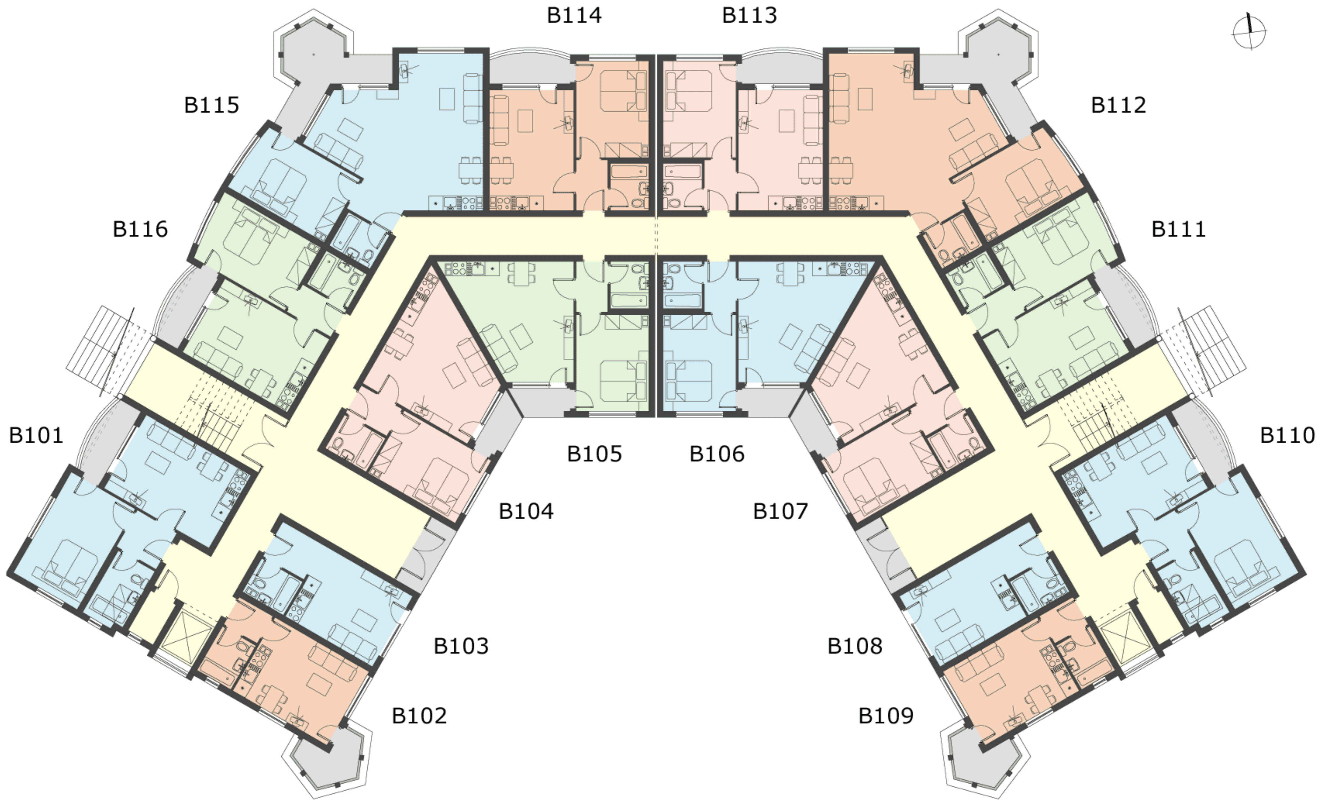
Block BII, floor 1 ( \pm 0.00 )
