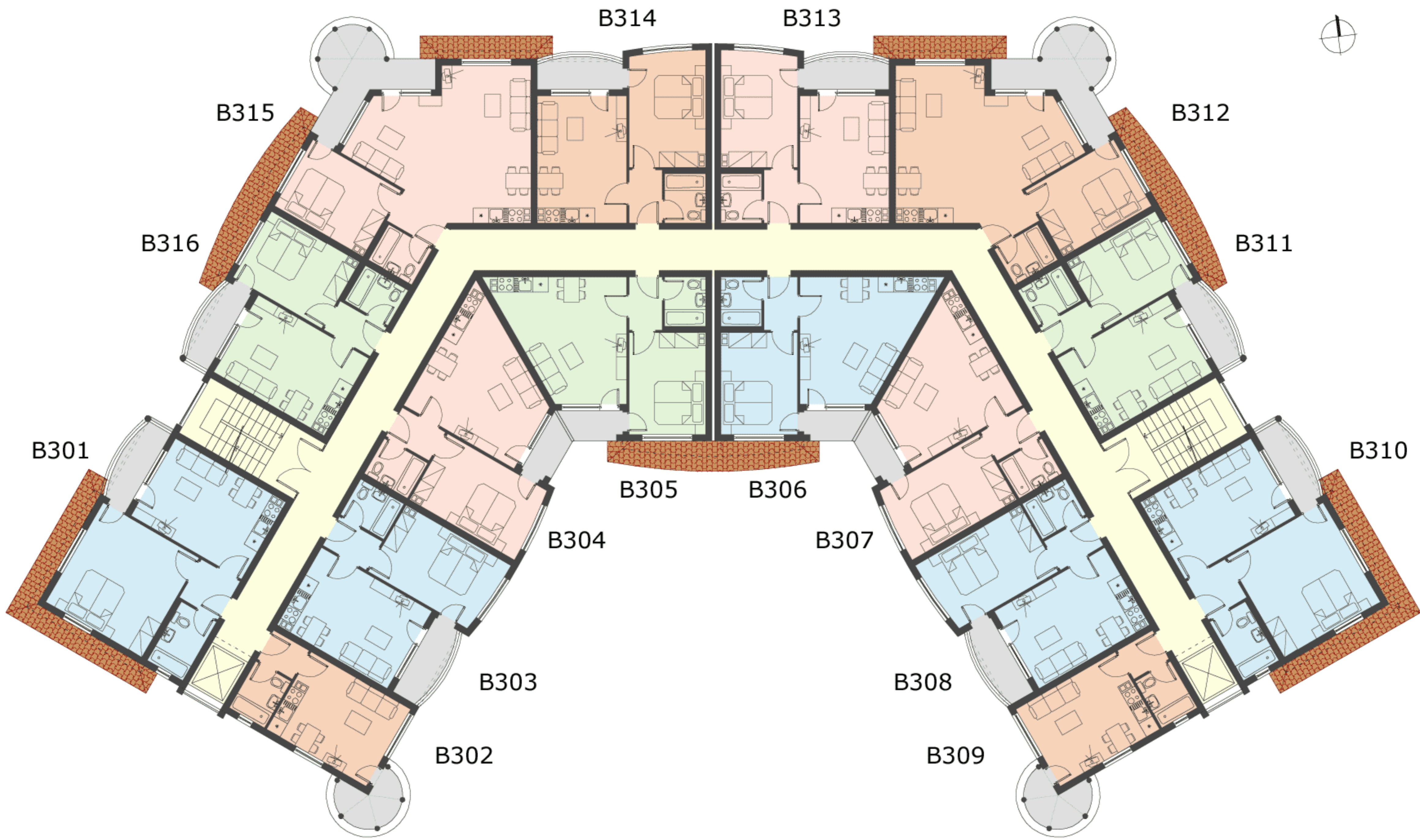
Block BII, floor 3 (+5.60)
